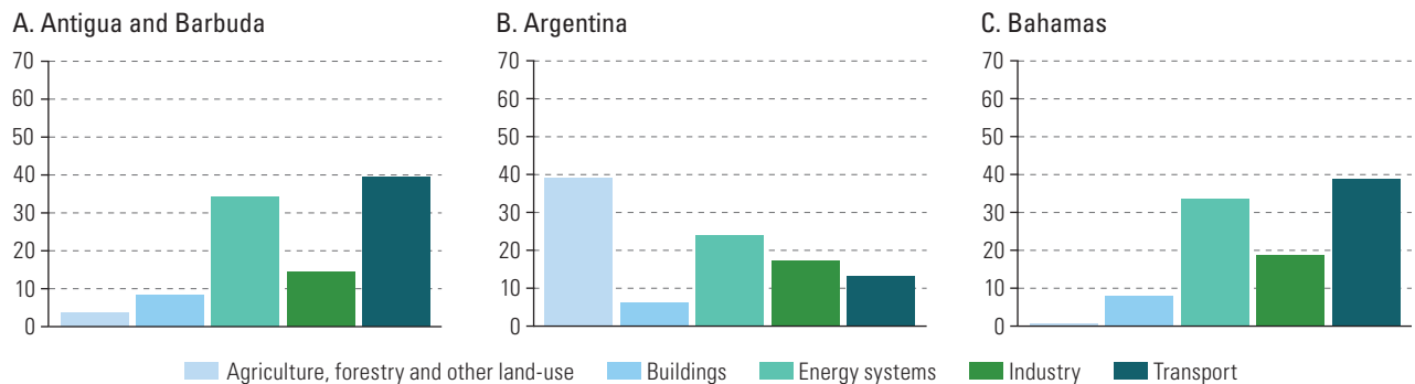
Figure 10 Latin America and the Caribbean (33 countries): greenhouse gas emissions by sector, 2019 (Percentages)
