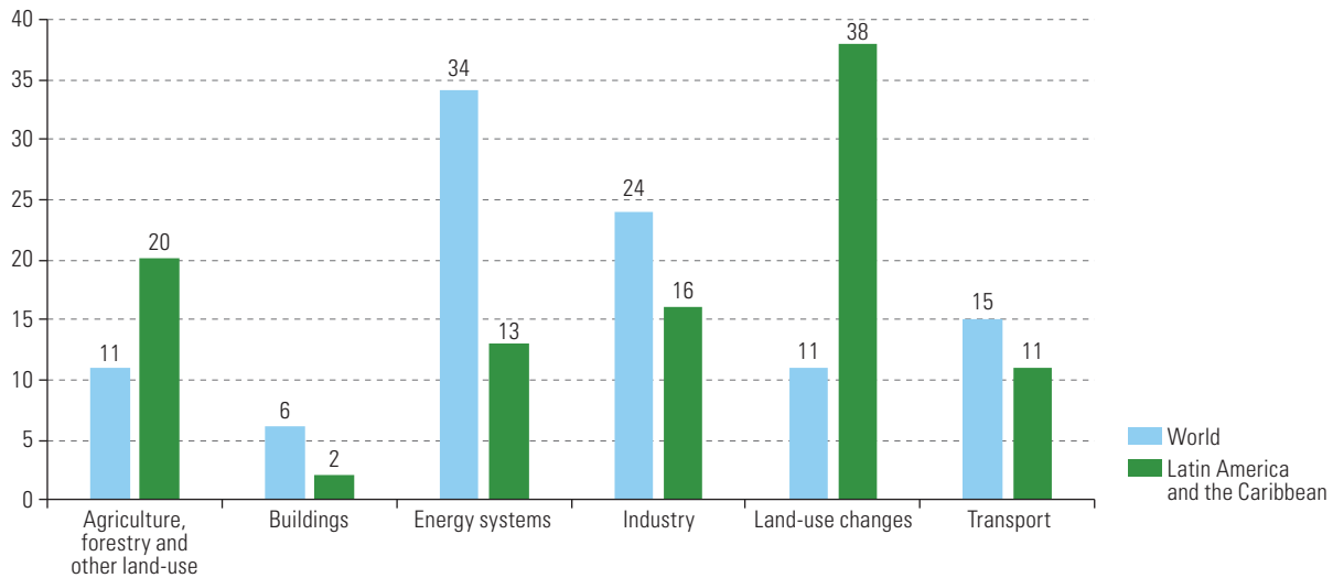
Figure 9 World and Latin America and the Caribbean: greenhouse gas emissions by sector, 2019 (Percentages)
