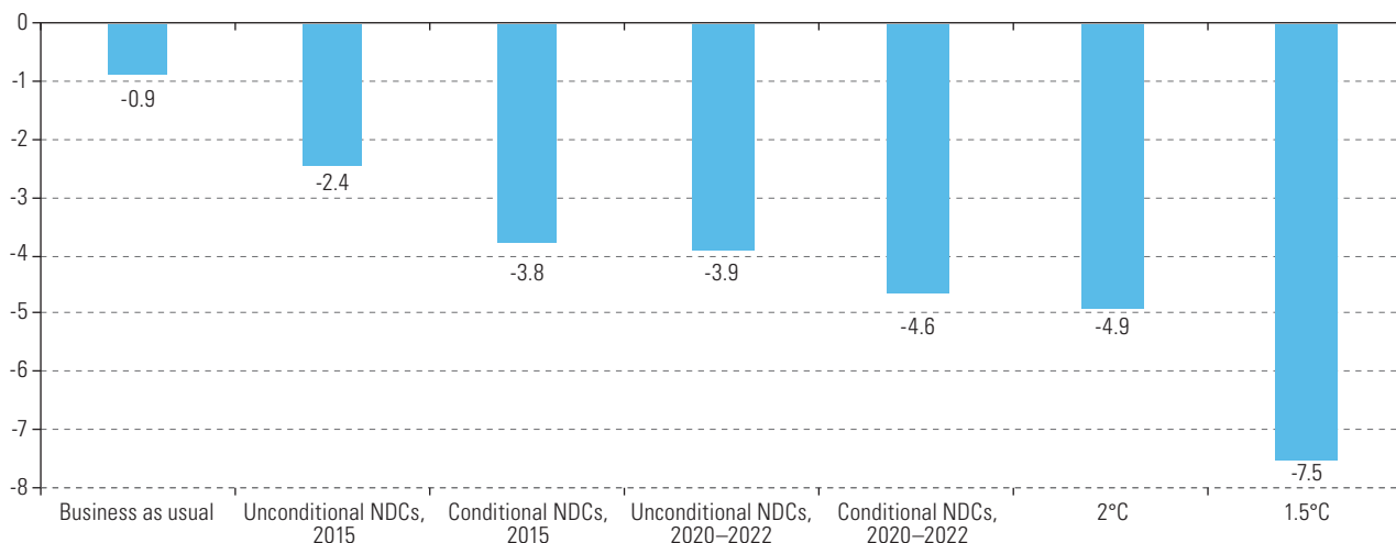
Figure 14 Latin America and the Caribbean: annual pace of decarbonization by scenario (Percentages)
