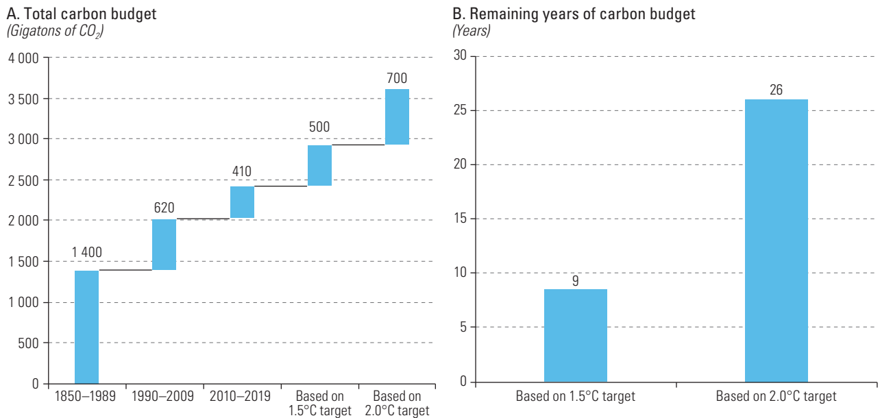
Figure 6 World: carbon budget by temperature target
