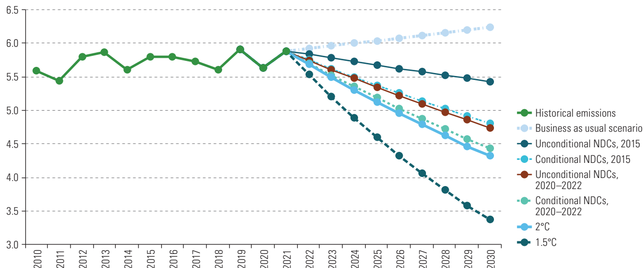
Figure 13 Latin America and the Caribbean: greenhouse gas emissions, 2010–2030 (Gigatons of CO 2 equivalent)
