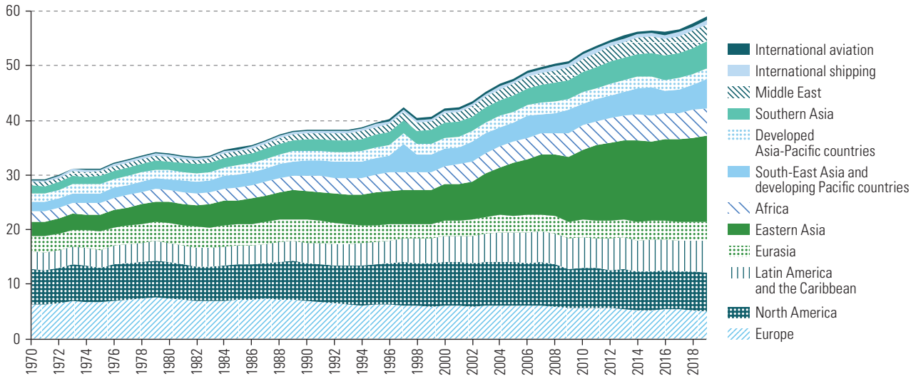
Figure 5 World: greenhouse gas emissions, 1970–2019 (Gigatons of CO 2 equivalent)
